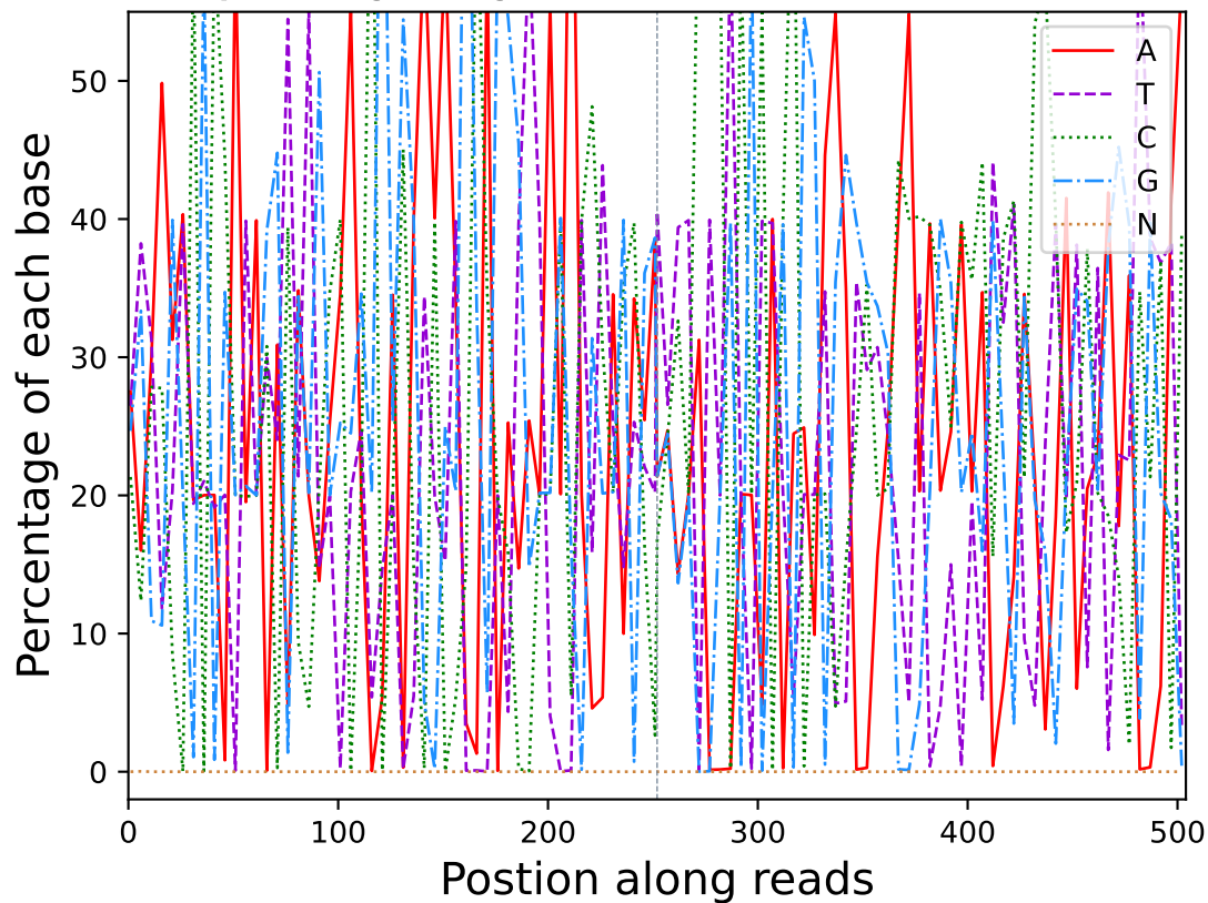
Base percentage along reads (R10416)
